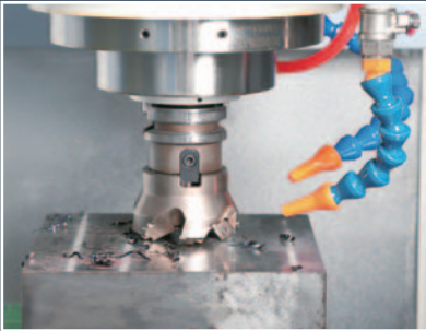
Face Milling
